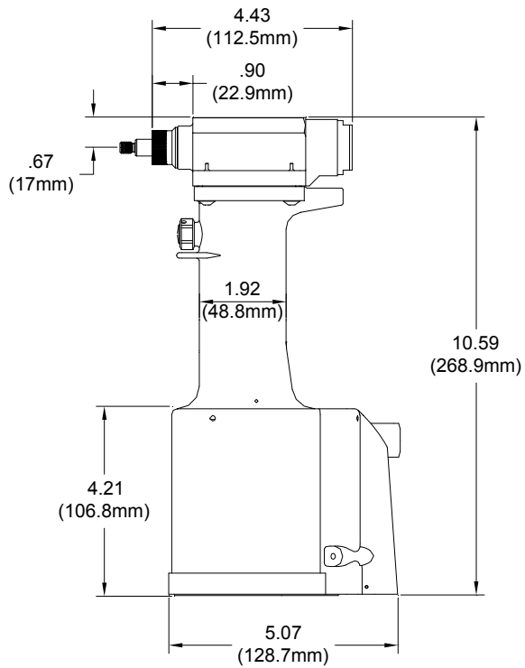
GBP715C
