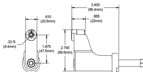
APPROXIMATE LONG DIMENSIONS
